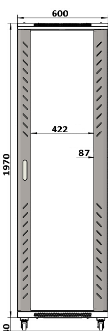
Front(Toughened glass)
